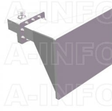
LB-340-15-C-7/16FSPO Standard Gain Horn Antenna 2.2-3.3GHz 15dB Gain 7/16(DIN) Female
